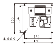
Controller mounting dimensions
