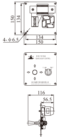
Controller mounting dimensions
