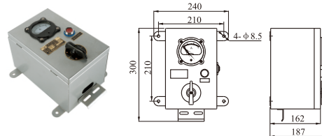
Control box of mercury-xenon lamp
