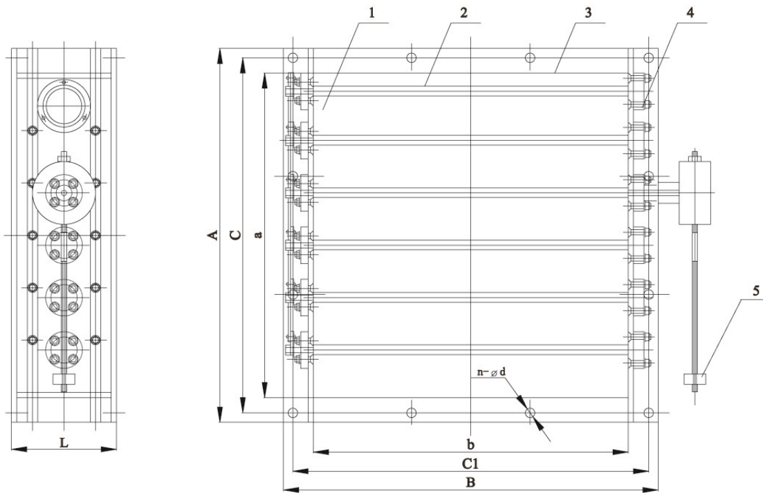
1.valve plate 2.valve body 3.flange 4.linkage mechanism 5.gravity hammer
